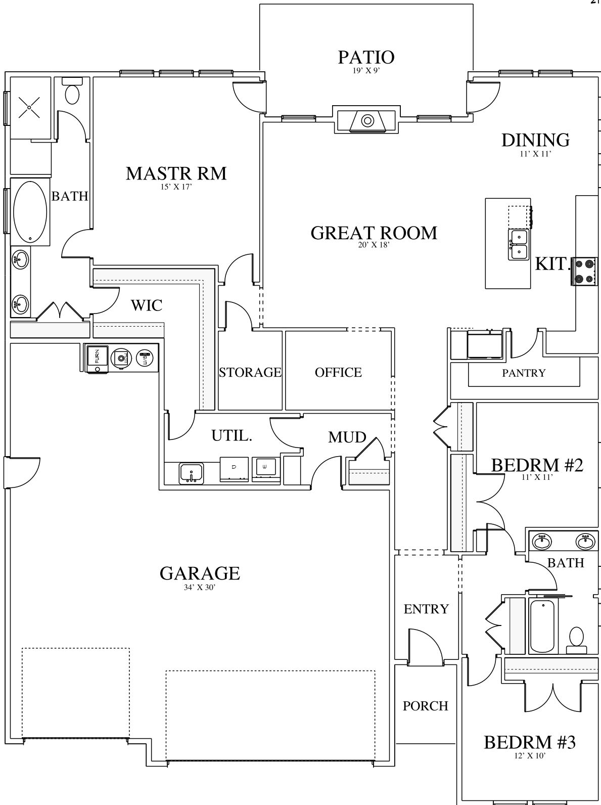
FLOOR PLAN 53' X 65'
