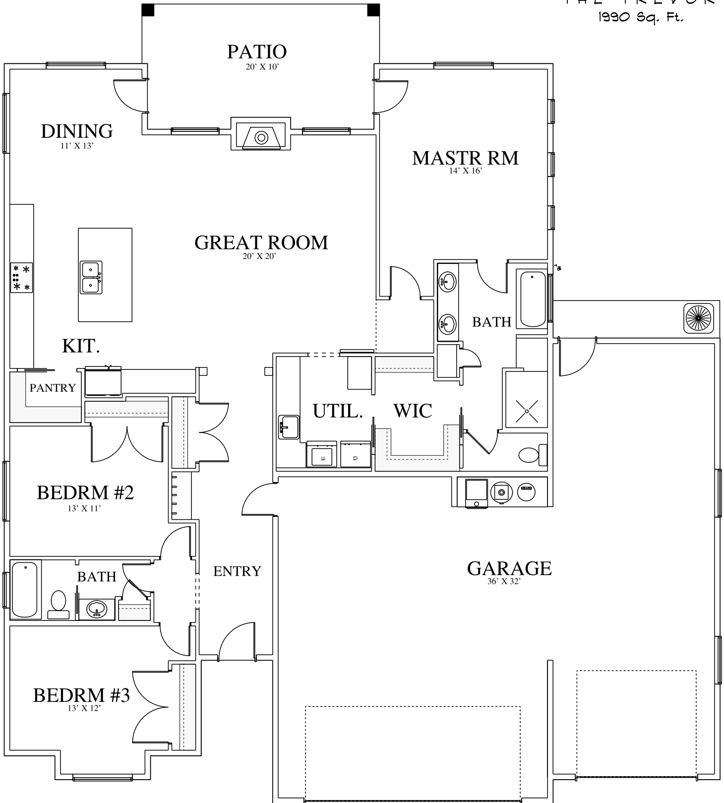
FLOOR PLAN 60' X 65'
